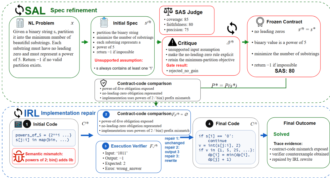
Figure 3: Case-study trace for LiveCodeBench problem 2883.
