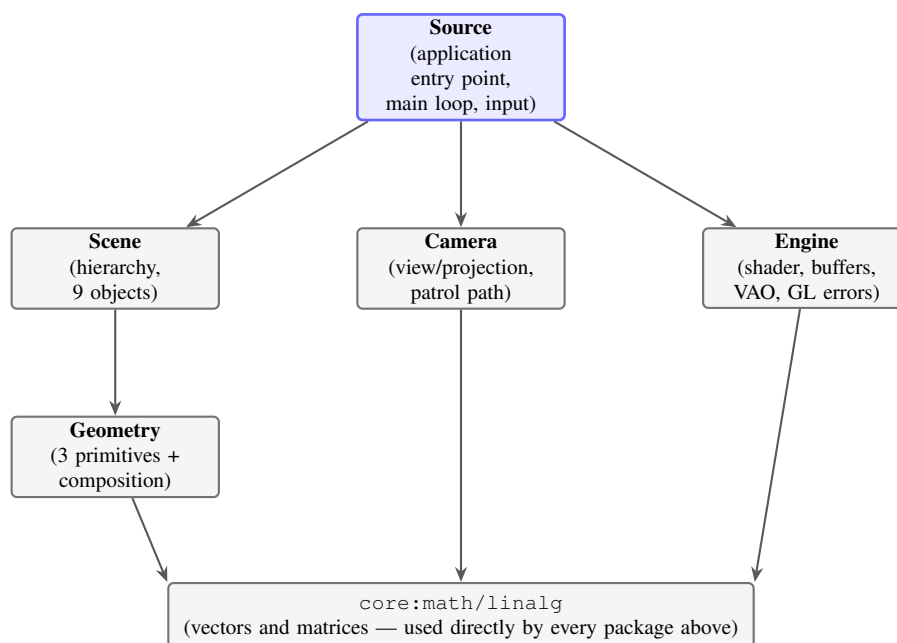
Figure 1: Package dependency structure. Engine and Geometry are theme-agnostic and know nothing about SENTINEL’s own objects; Scene and Camera sit above them, and the Source application ties everything together. Two minor edges are omitted for readability: Geometry also depends on Engine for its GPU buffer types, and Scene depends on core:math/linalg directly in addition to via Geometry .
