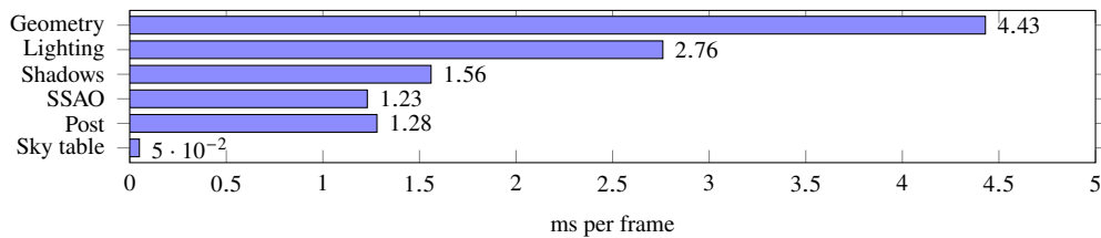
Figure 4.1: GPU time per pass (total 11.28 ms of the 16.7 ms budget).
