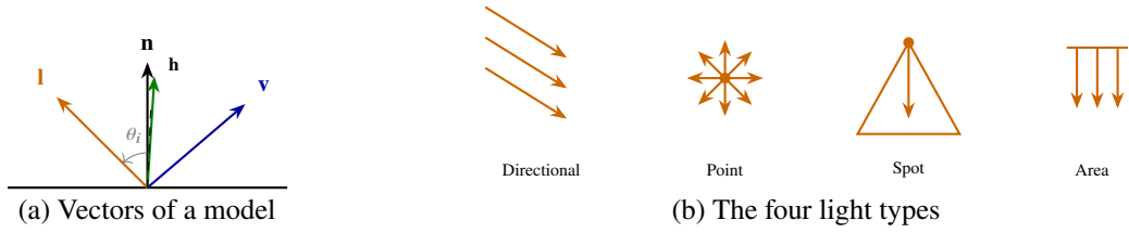
Figure 3.6: The geometry of lighting: surface normal, light, view and half vectors; sun, lamp, spotlight and rectangular panel.
