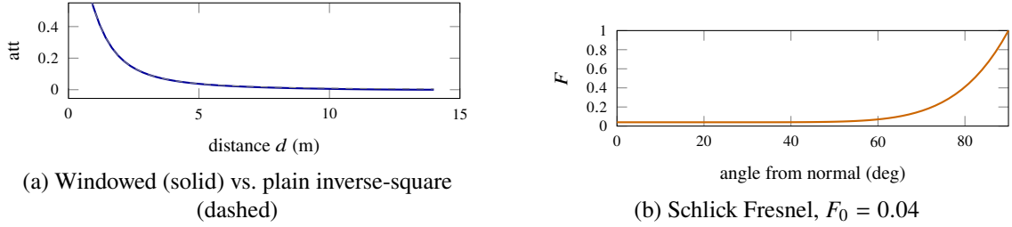
Figure 3.8: Two curves behind the lighting: distance falloff and glancing-angle reflection.
