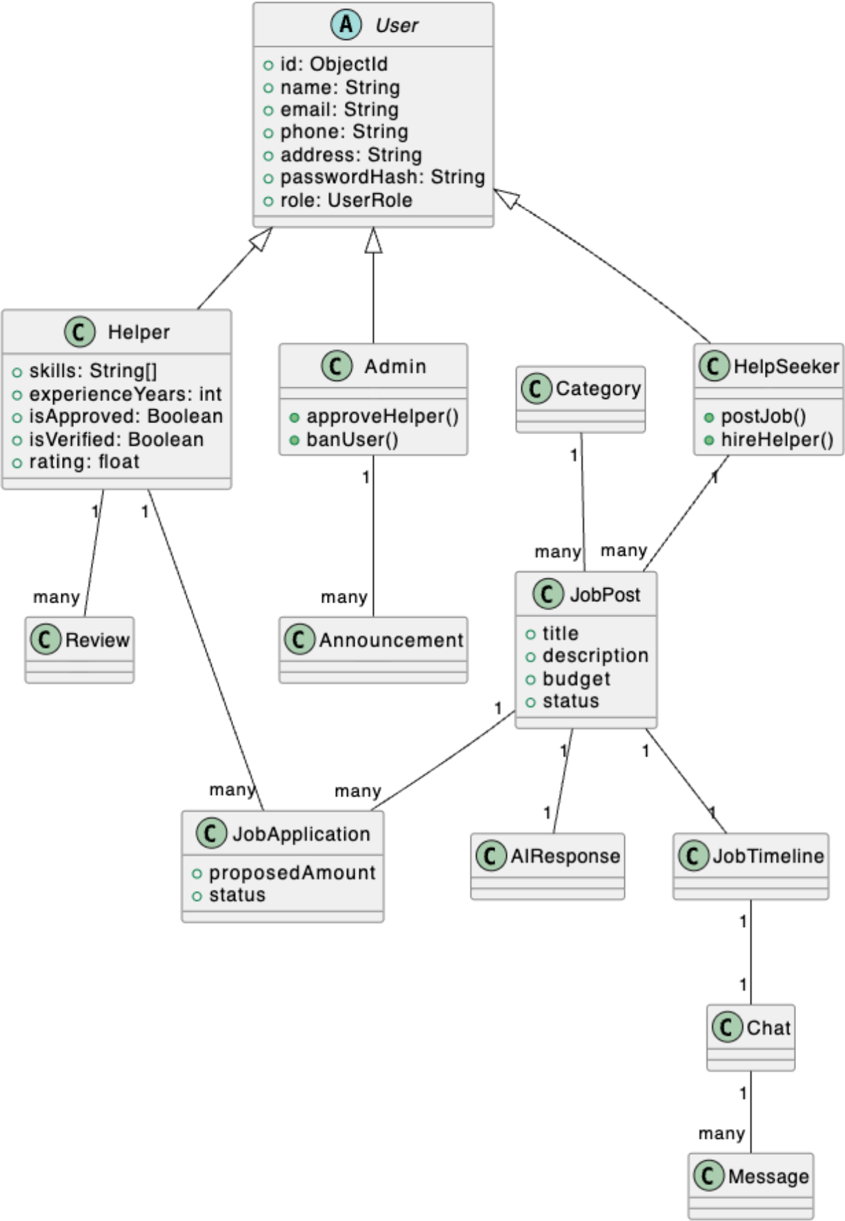
MistriHub - Full Class Diagram
