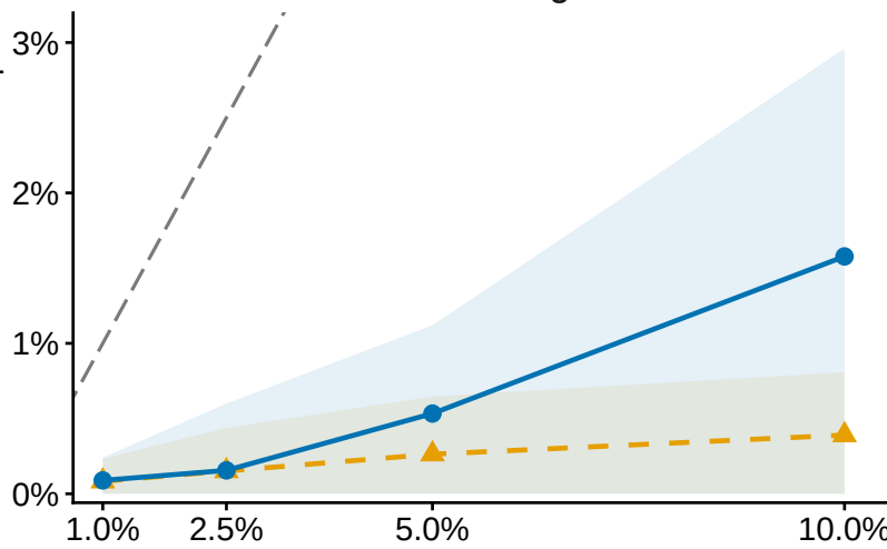
Difficult designs
