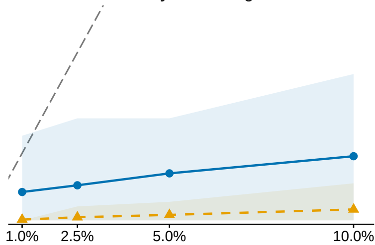
Partially linear designs
