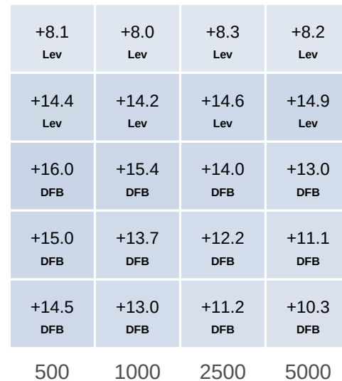
Bad leverage
