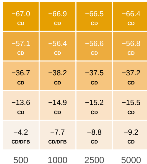
Good leverage
