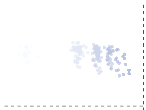
Mixed normal
