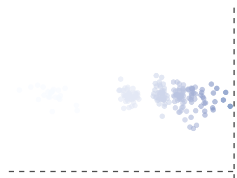
Skewed t
