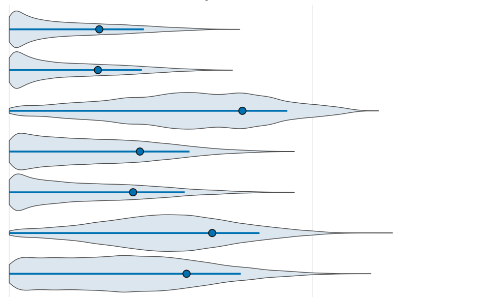
Response outliers
