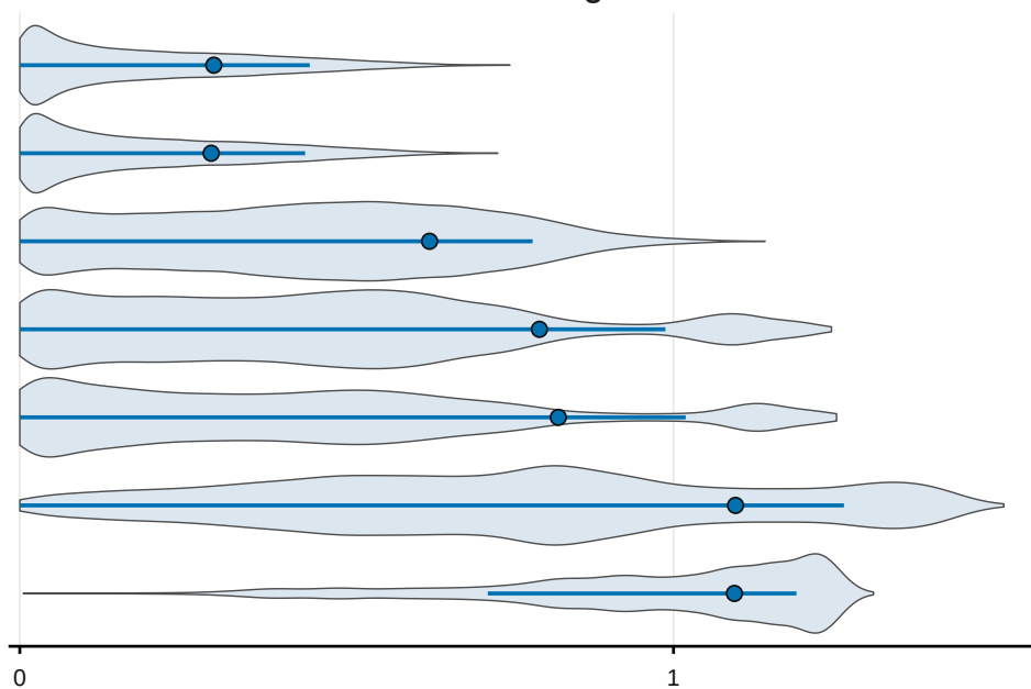
Bad leverage
