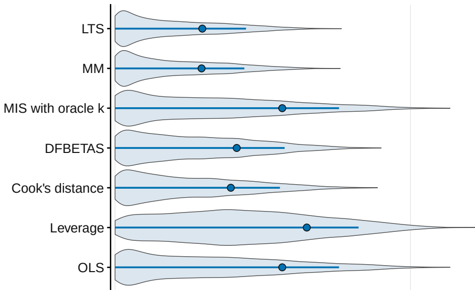
No contamination
