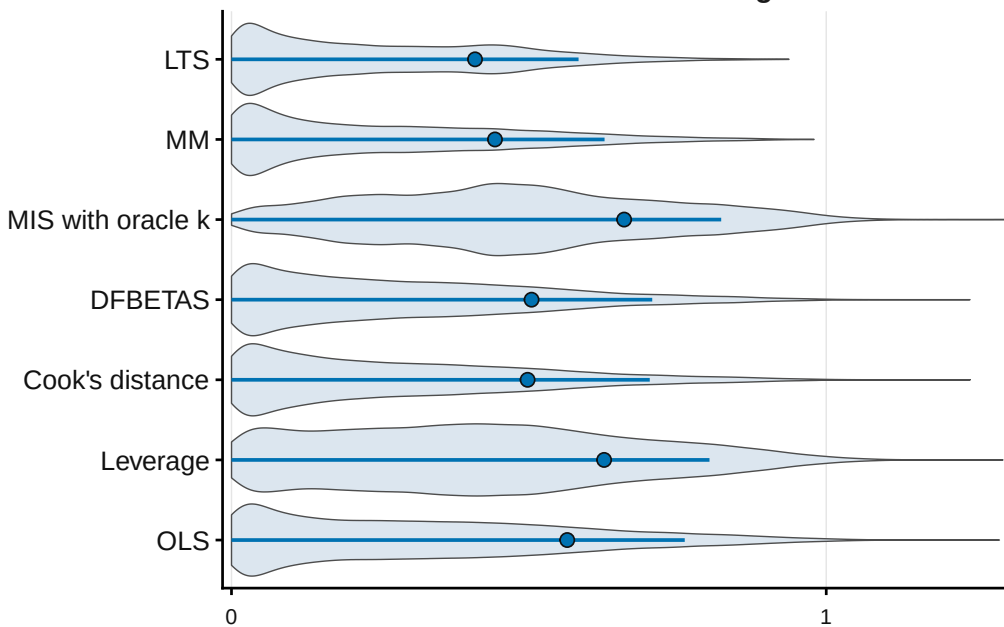
Good leverage
