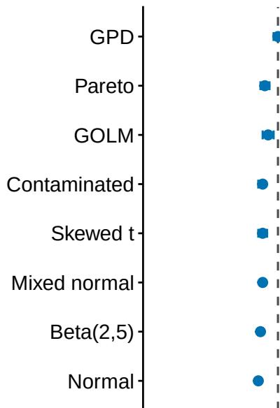
\log_2 \text{leverage detected} / \text{injected}
