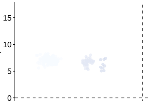
Normal
