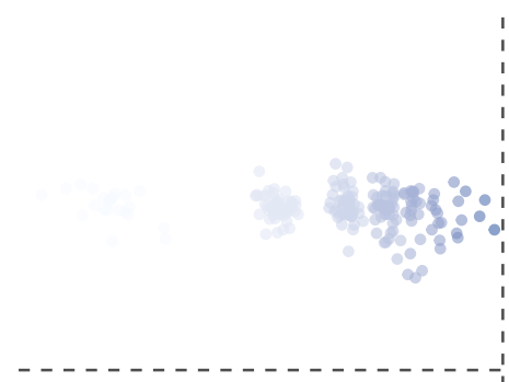
Skewed t
