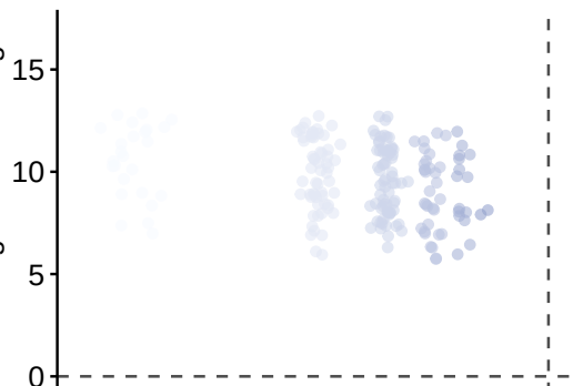
Contaminated
