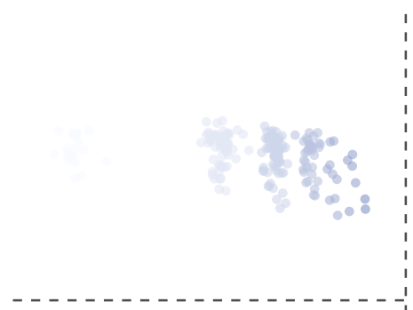
Mixed normal
