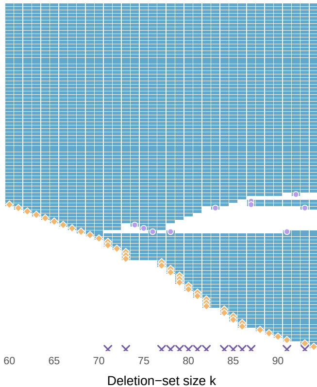
Influential-set turnover
