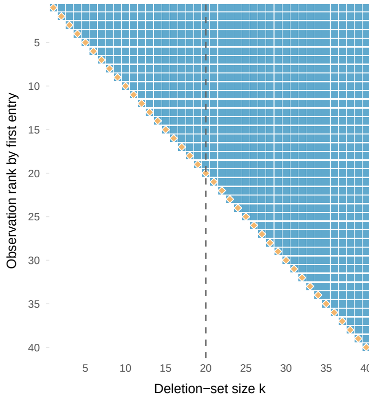
Stable-core accumulation
