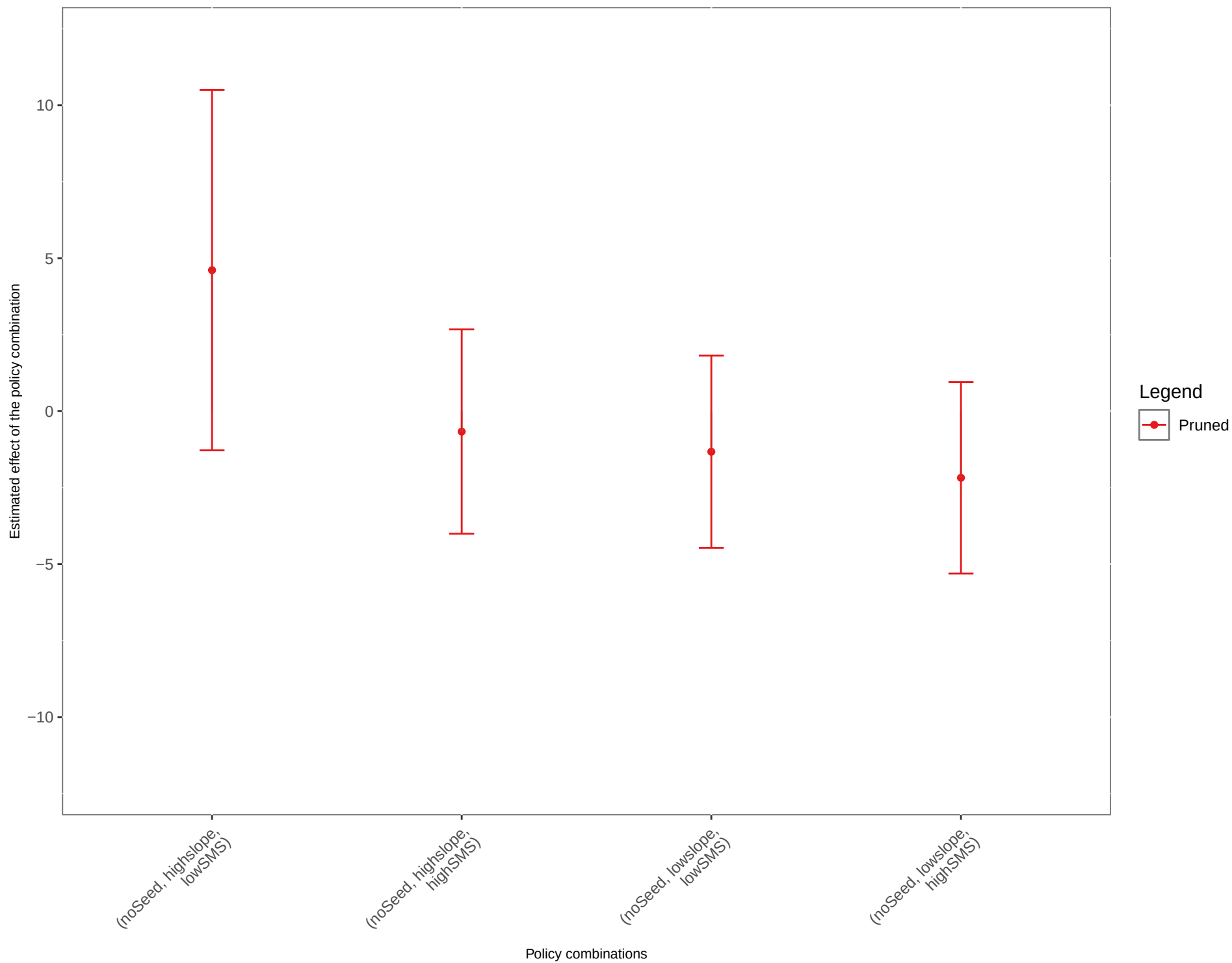
Results of the naive OLS for the treatment profile (any slope Incentive, noSeed, any Reminder)
