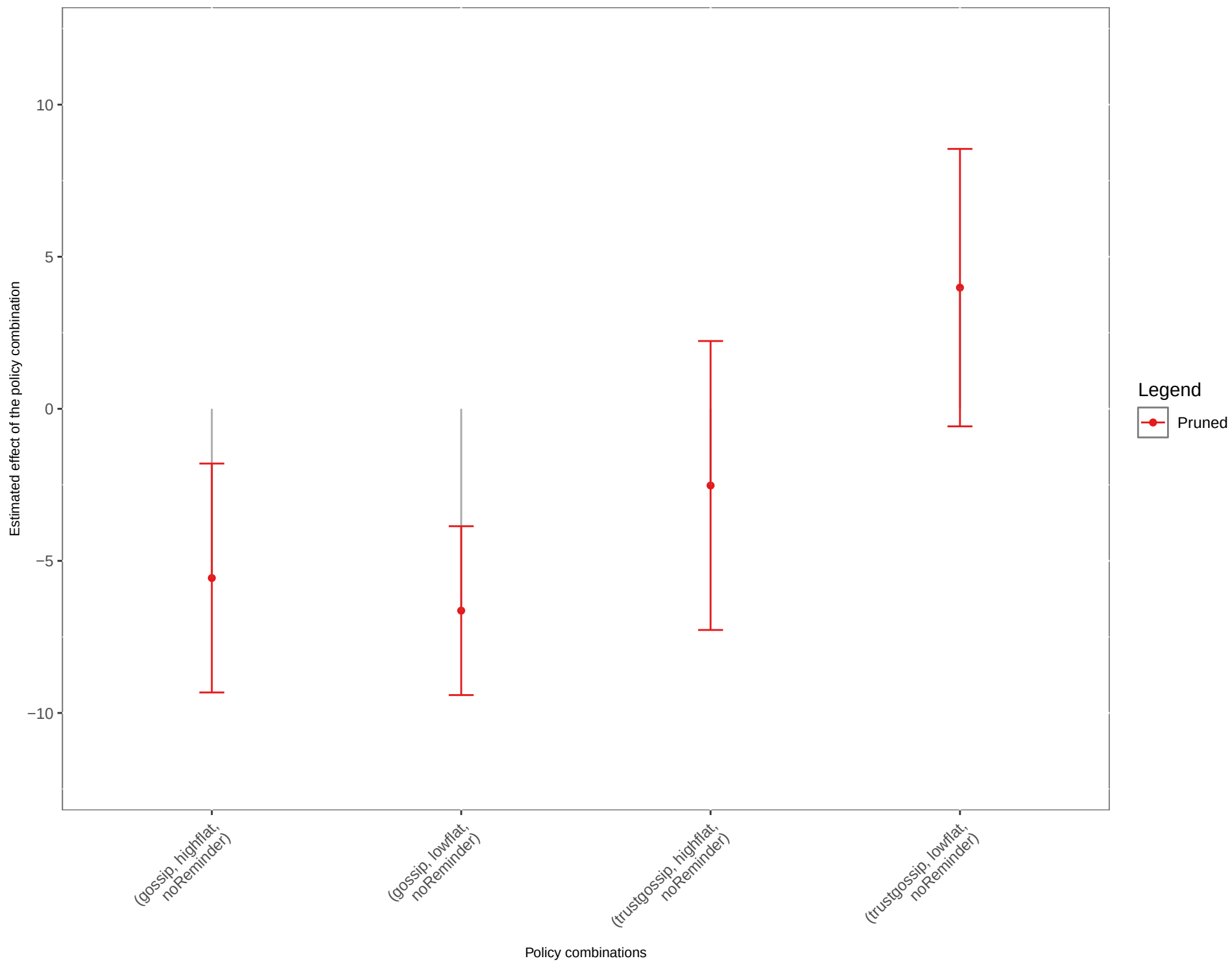
Results of the naive OLS for the treatment profile (any flat Incentive, any gossip, no Reminder)
