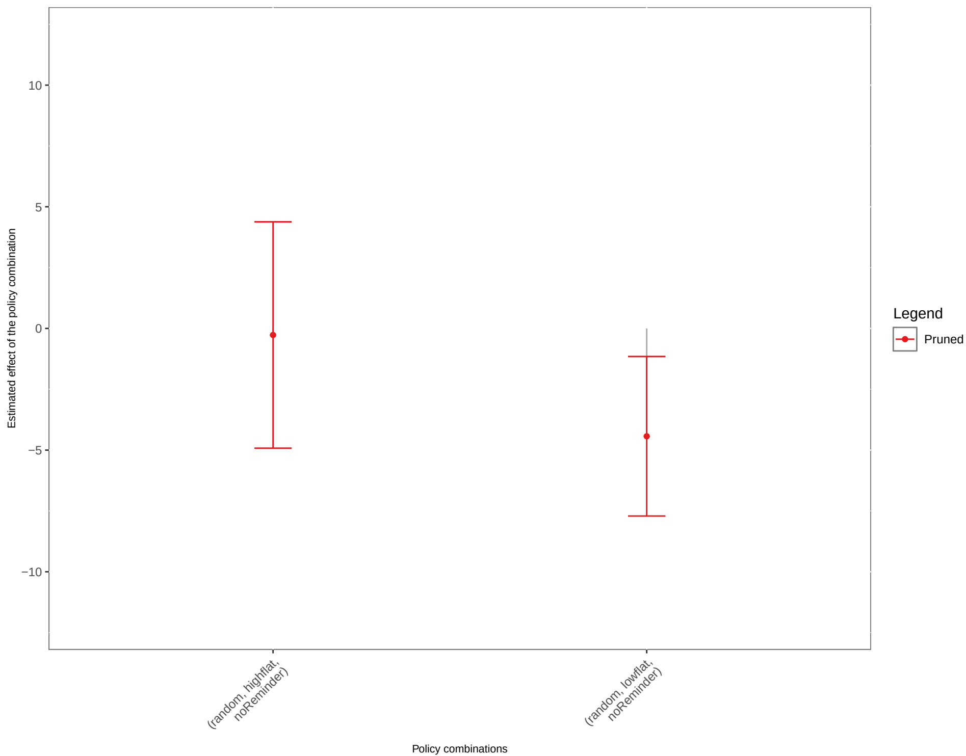
Results of the naive OLS for the treatment profile (any flat Incentive, random, no Reminder)
