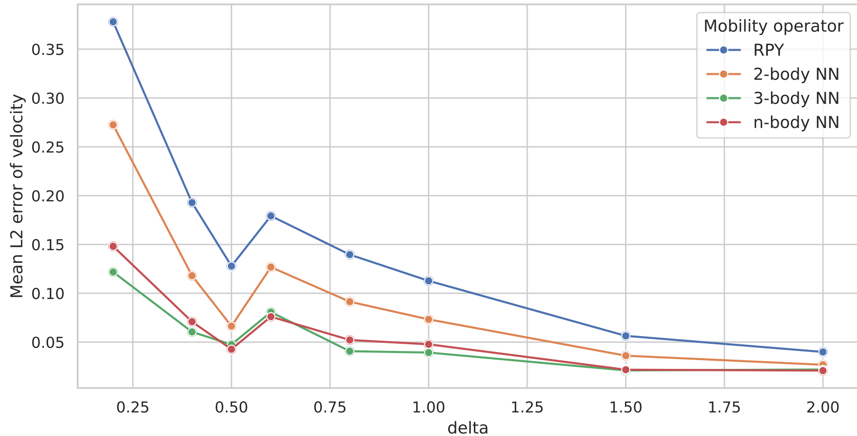
Grand mobility accuracy vs operator type (varying delta)
