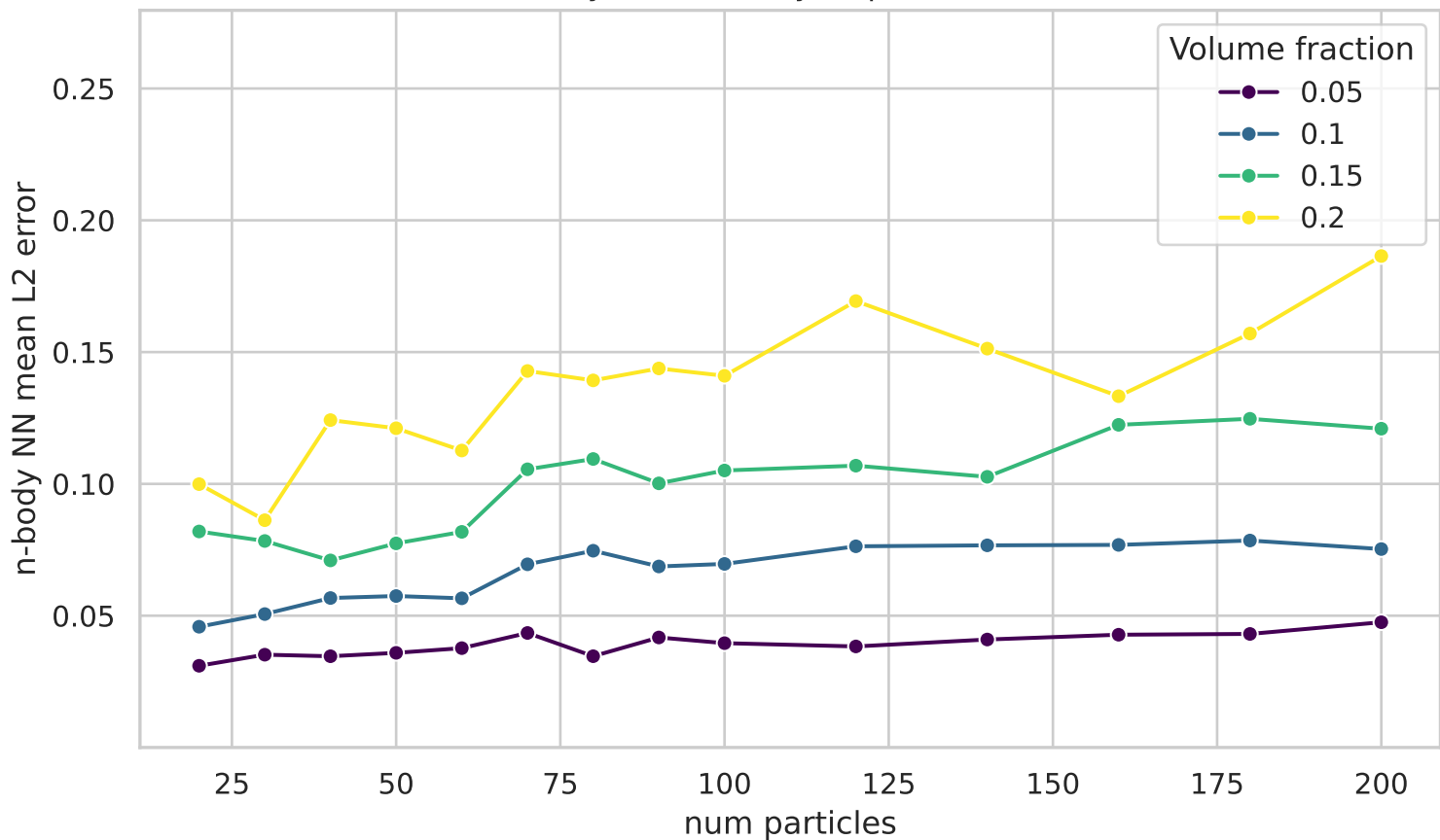
n-body NN accuracy vs particle count
