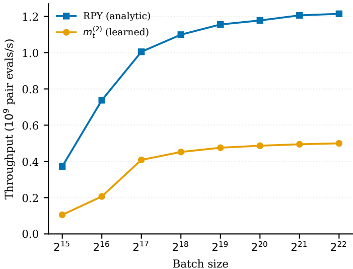
Two-body pair kernel
