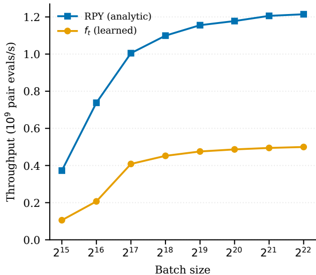
(a) Two-body pair kernel
