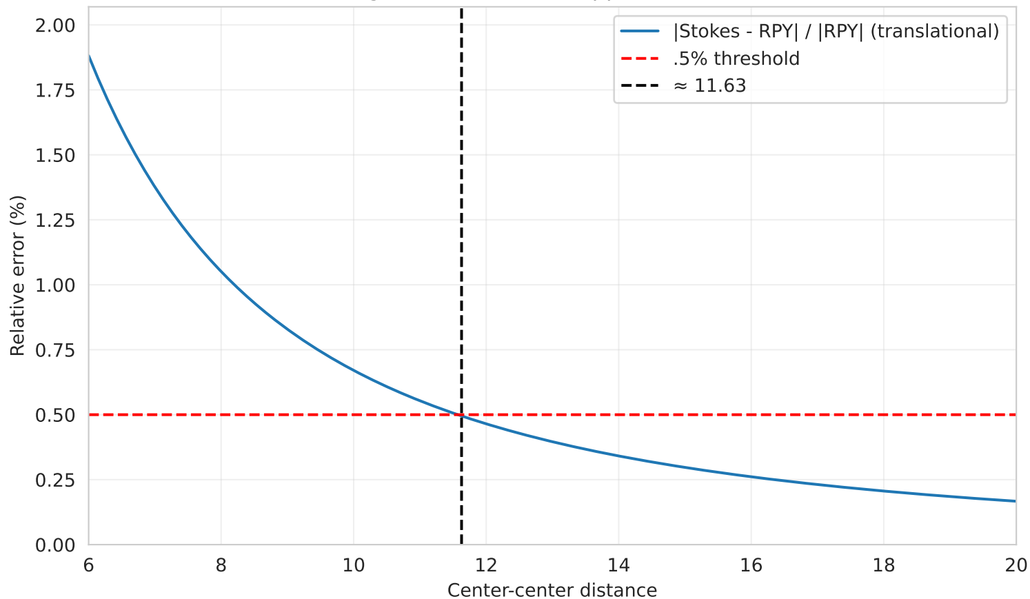
Convergence of Stokeslet approximation to RPY
