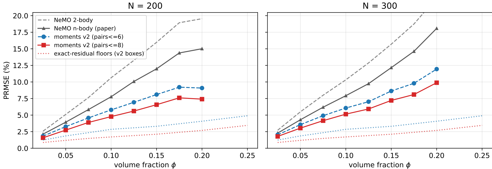
Figure 3 protocol: pair_cutoff 6 vs 8 (moments v2, all neighbours, r_c = 8 )
