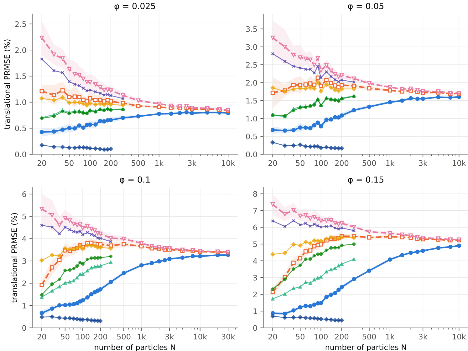
Uniform gravity, torque-free spheres: error vs N (seed mean, \pm 1 std band on the main curves)
