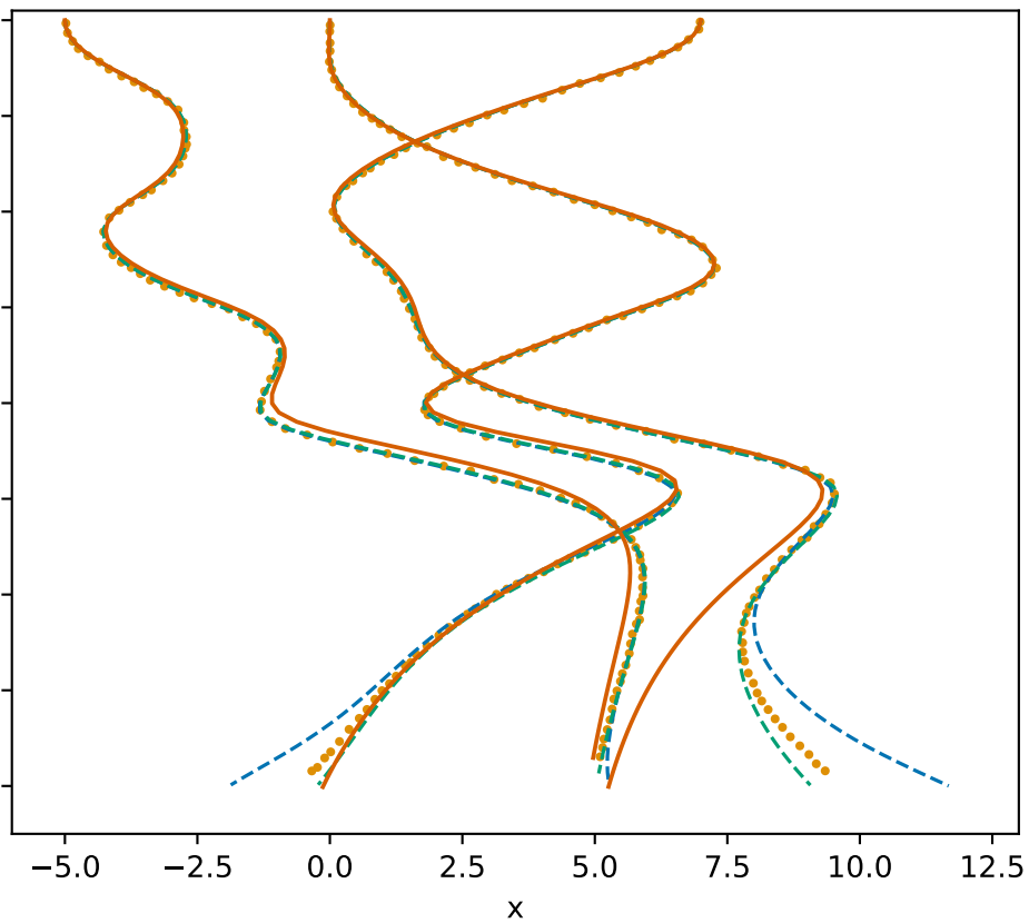
learned two-body M_{2b}
