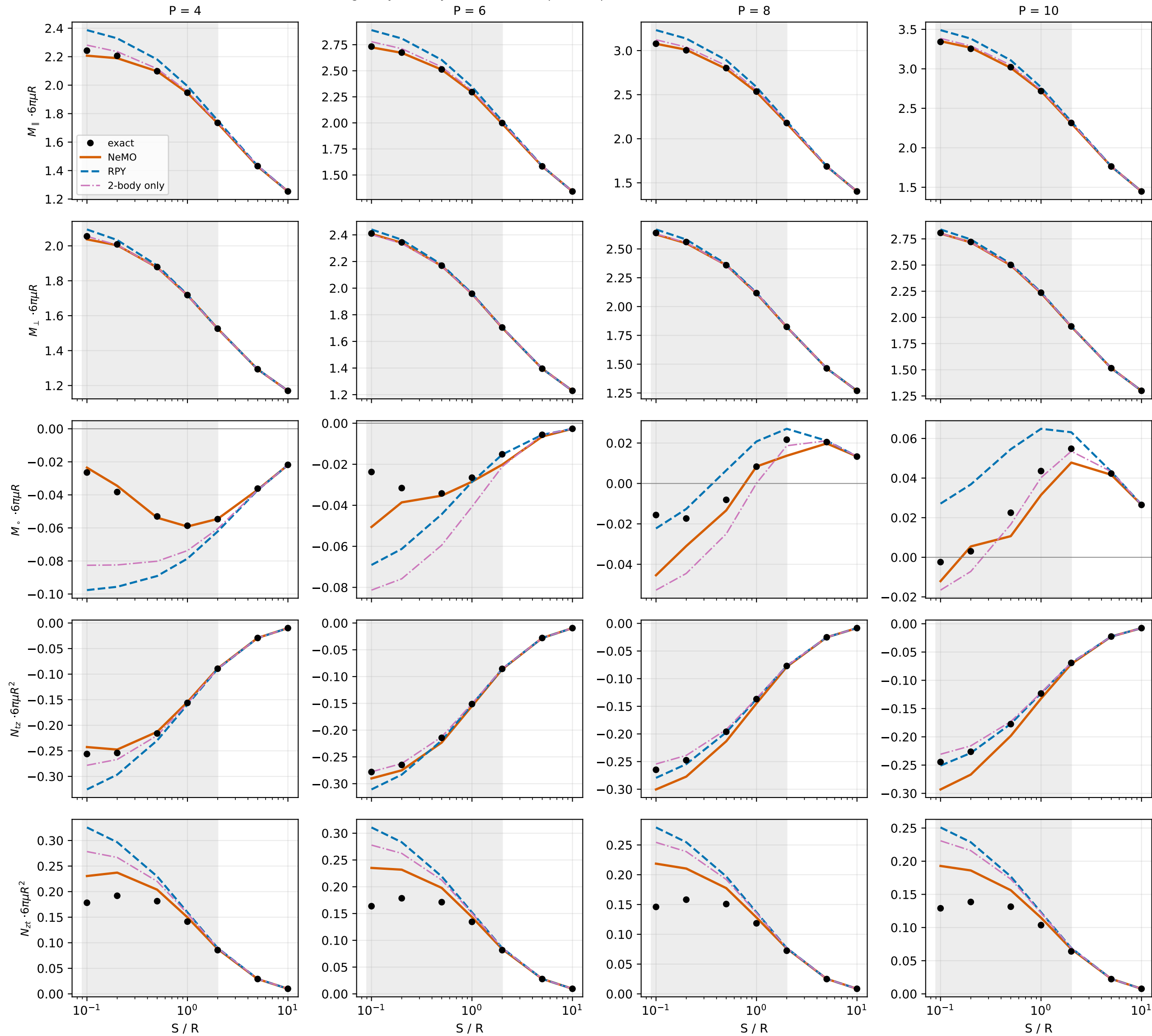
Ring-array mobility coefficients vs sphere separation (shaded: near field, S \leq 2R )
