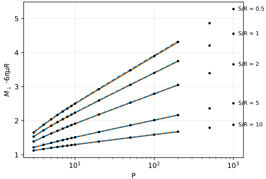
Global ring mobility vs number of spheres
