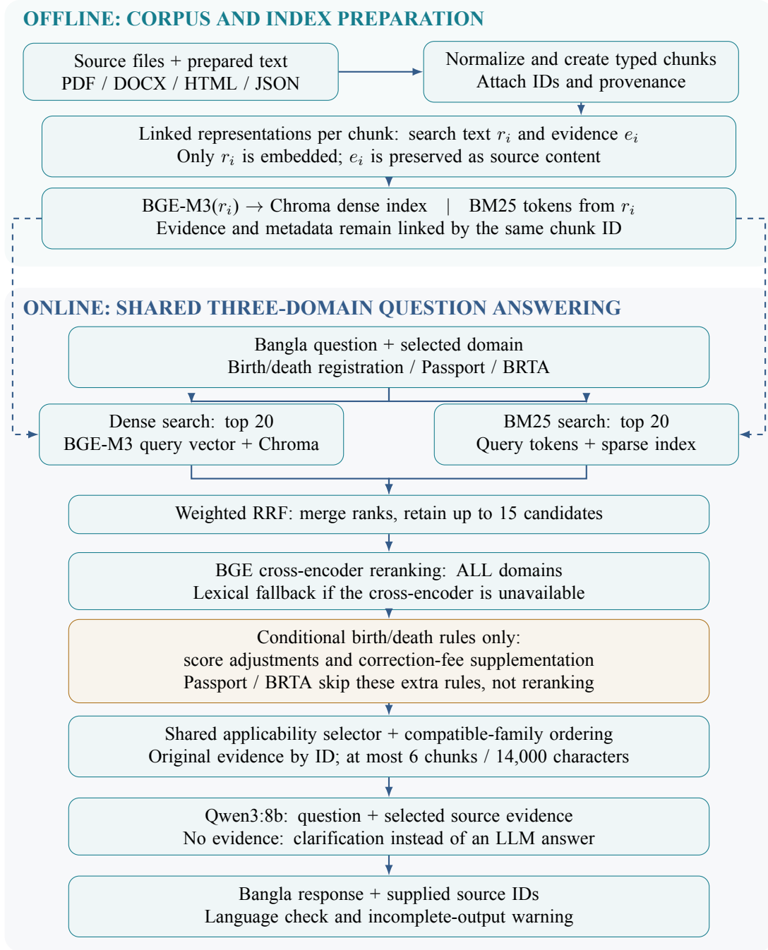
Figure 4.1: Current CivicRAG architecture, redrawn from the P2 offline/online organization and updated for three domains. Dashed arrows indicate index access. The gold box distinguishes domain-specific rules from shared reranking. The selected-evidence route bypasses the legacy controlled-answer branch.
