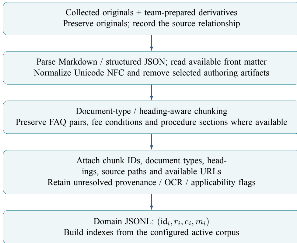
Figure 4.2: Source-preserving preparation of the active corpus: original materials remain available while normalized derivatives are organized into identifiable retrieval units. Separate cleanup candidates are not substituted for the evaluated corpus.
