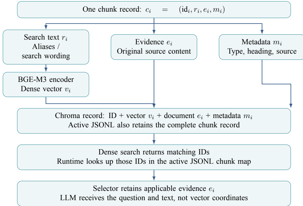
Figure 4.3: How answer evidence remains connected to a vector without being generated by the database. BM25 is a separate index of r_i , omitted here to isolate the dense-storage link. All arrows entering storage denote stored fields, not additional embeddings.
