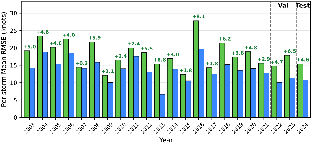
Dataset Partitioning (2003-2024)
