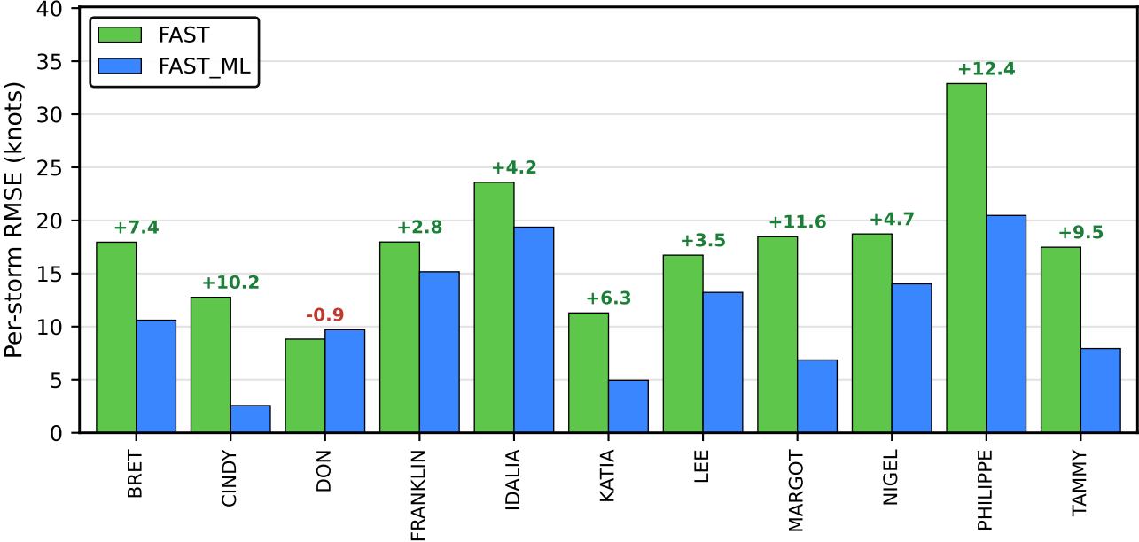
2023 (Validation)
