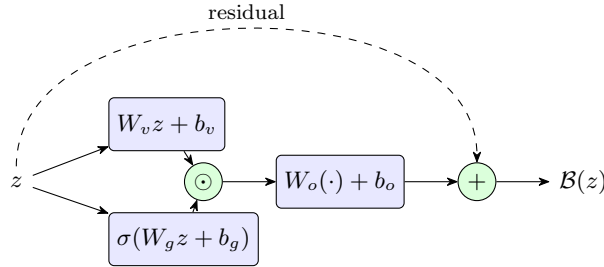
Figure 2: The residual GLU block \mathcal{B} (Eq. 7): a value branch W_v z and a sigmoid gate \sigma(W_g z) are multiplied elementwise ( \odot ), projected by W_o , and added back to the input (the residual skip). In trunk variant A one such block (its own d \times d weights) follows the input projection, before the residual MLP stack.
