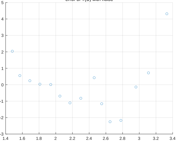
error of T(U) with noise
