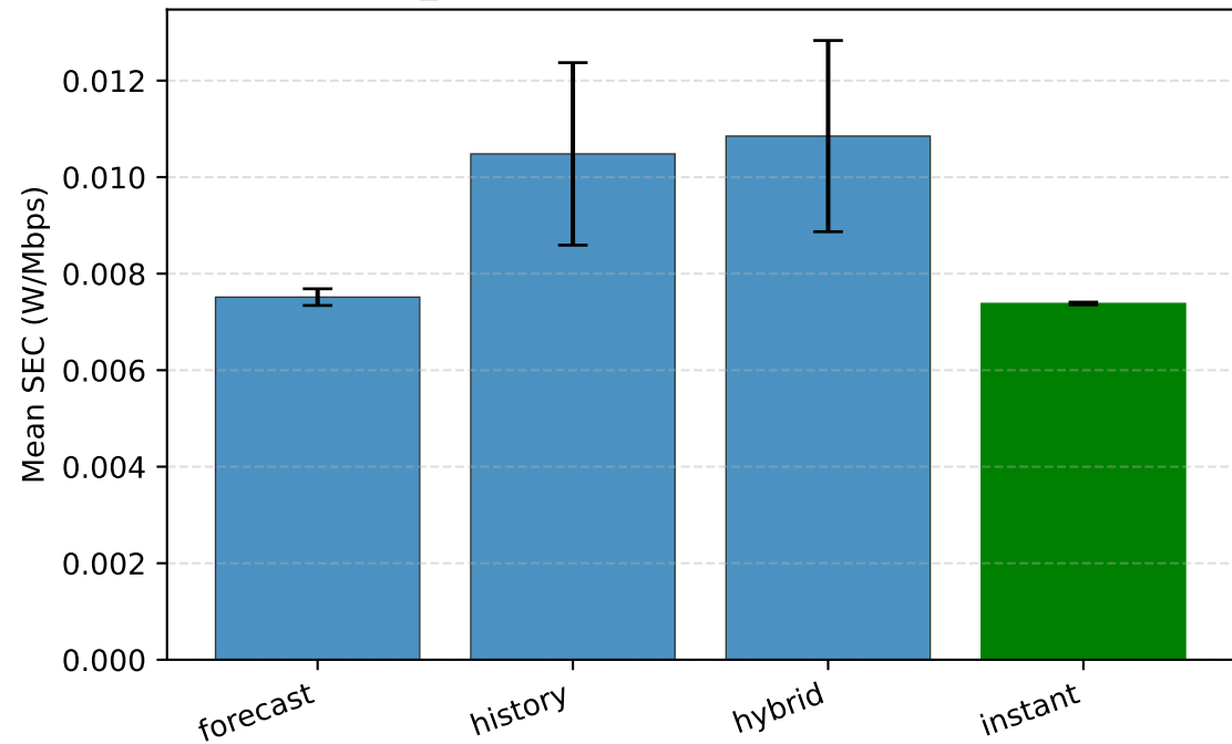
A2_observation: Mean SEC (W/Mbps)
