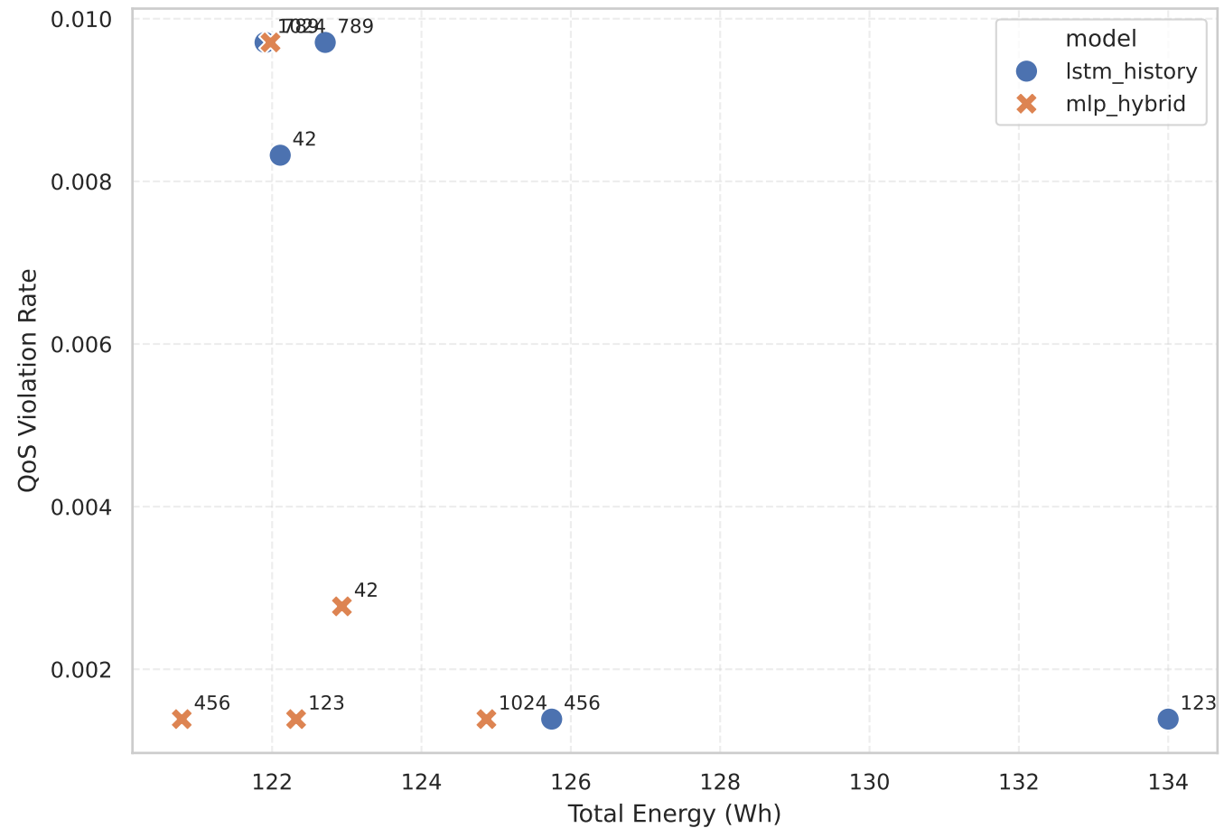
B2 Trade-off: Total Energy vs QoS Violation
