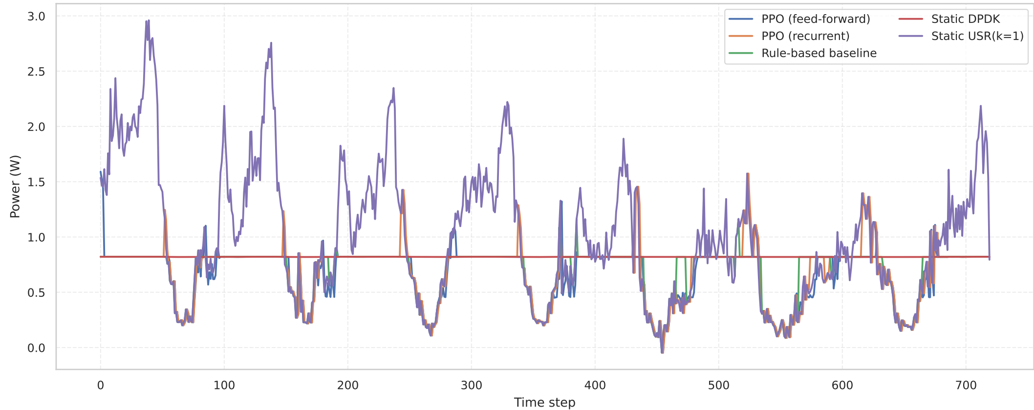
Interval-averaged power over test horizon
