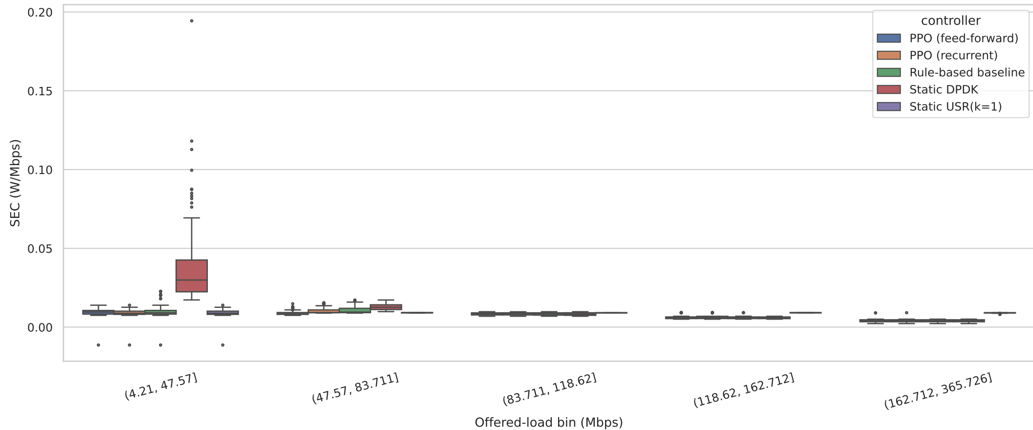
Specific energy consumption by load bin
