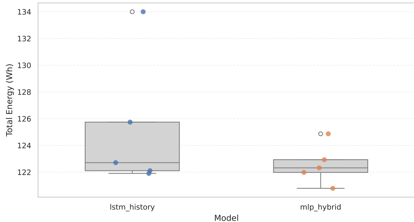
B2 Distribution: Total Energy by Model
