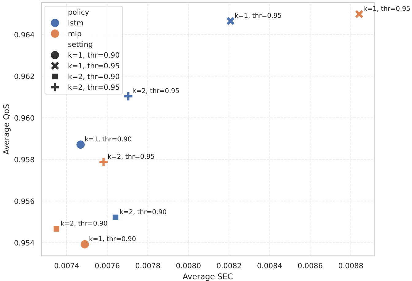
D1 Tradeoff: Avg SEC vs Avg QoS
