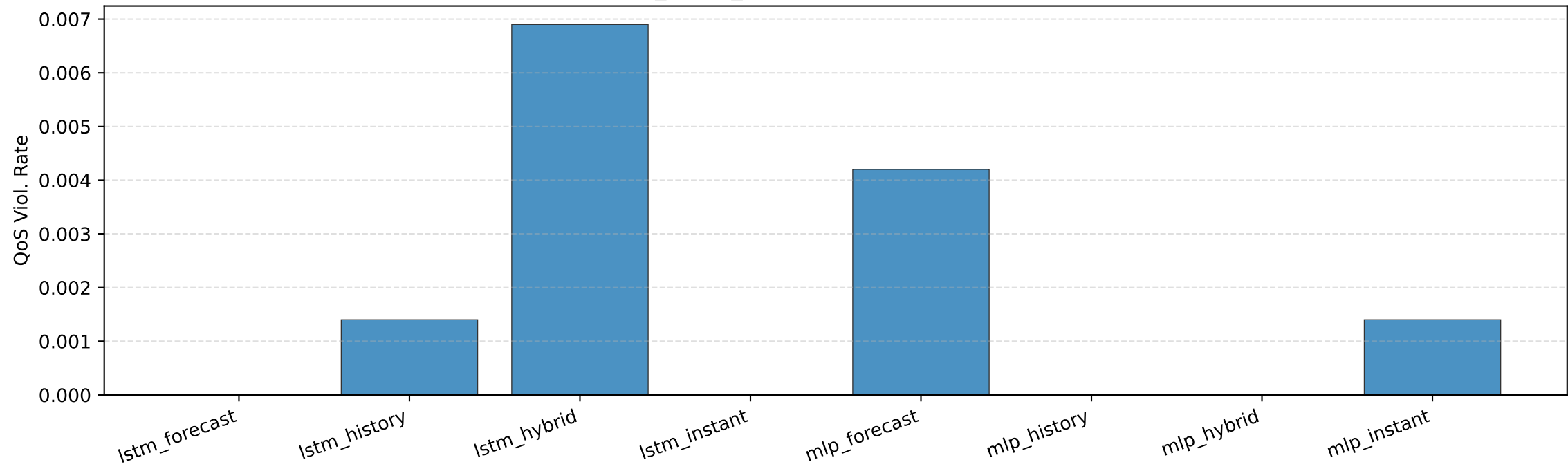
A1_policy_observation: QoS Viol. Rate
