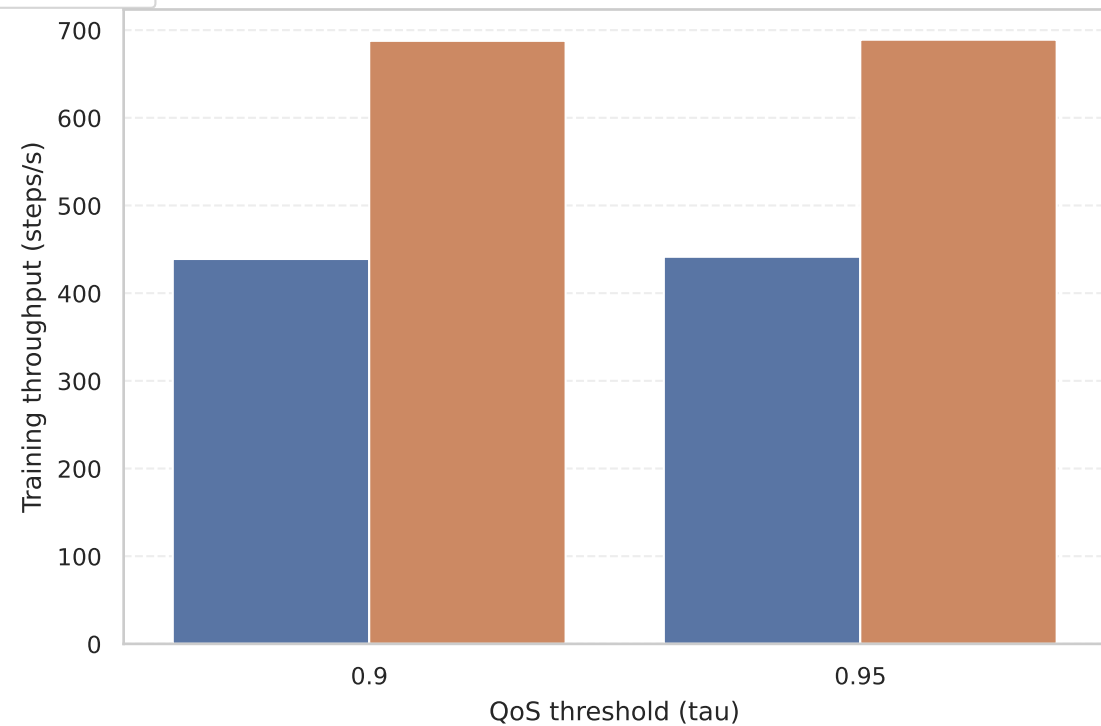
Training throughput by policy and threshold
