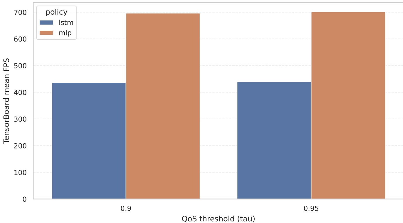
TensorBoard throughput by policy and threshold
