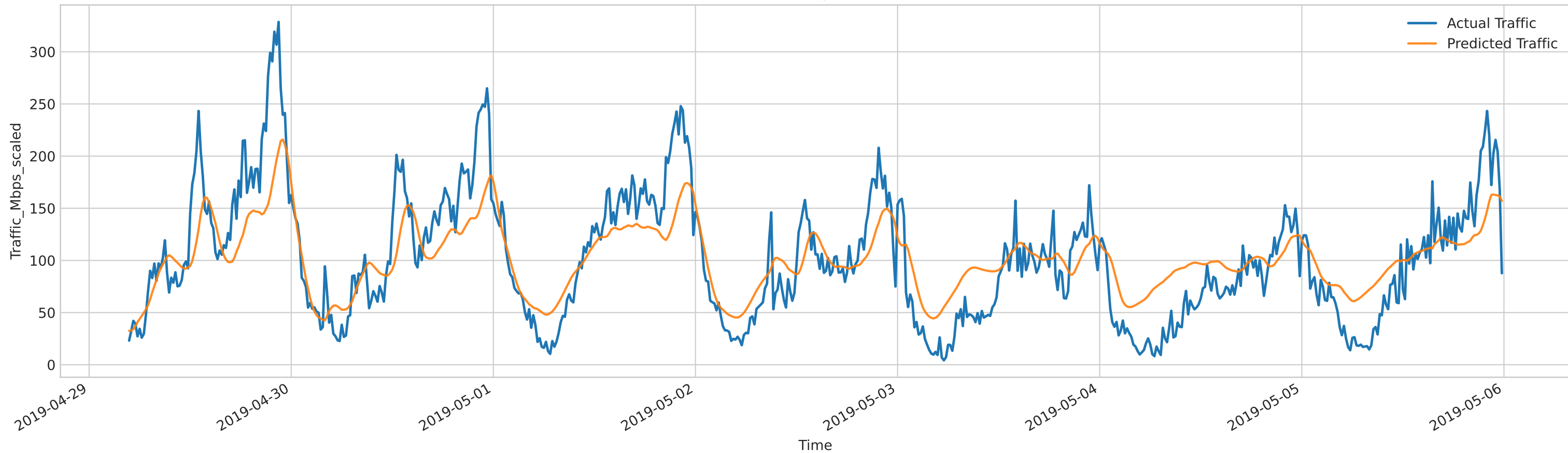
Traffic Prediction on Held-out Split (RMSE=36.15, R^2=0.638 )
