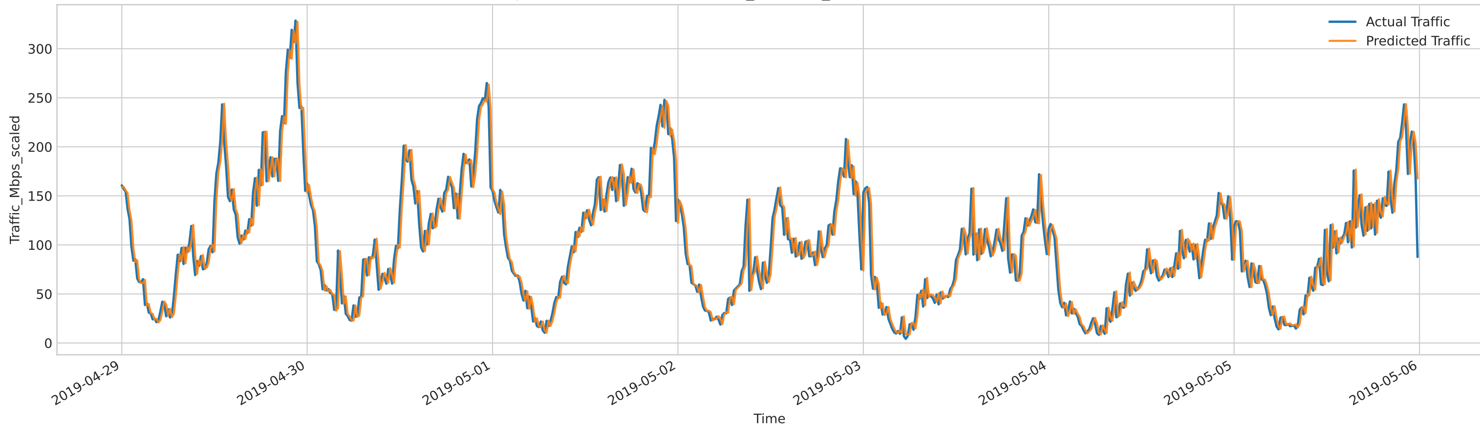
Best Improved Traffic Predictor: delta_calendar_huber (RMSE=19.12, R2=0.898)
