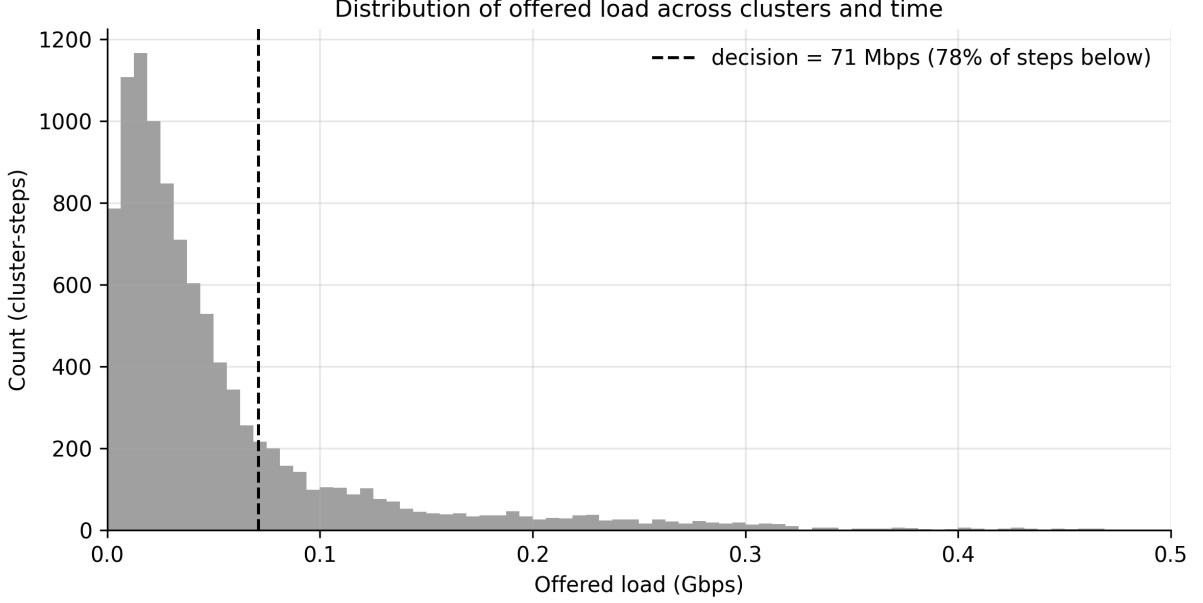
Figure 1.5: Distribution of calibrated offered load across all clusters and time windows. About 78 % of cluster-steps lie below the derived decision threshold (dashed), i.e. in the regime where USR-UPF is the safe and cheaper action.
