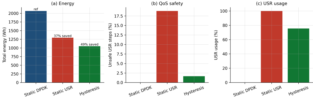
Figure 1.7: Aggregate comparison of the non-learning controllers. (a) Total energy (with saving vs. static SD-CORE DPKK annotated); (b) unsafe USR-UPF rate; (c) USR-UPF usage. Hysteresis saves the most energy and is nearly always safe, whereas static USR-UPF is cheap but frequently unsafe.
