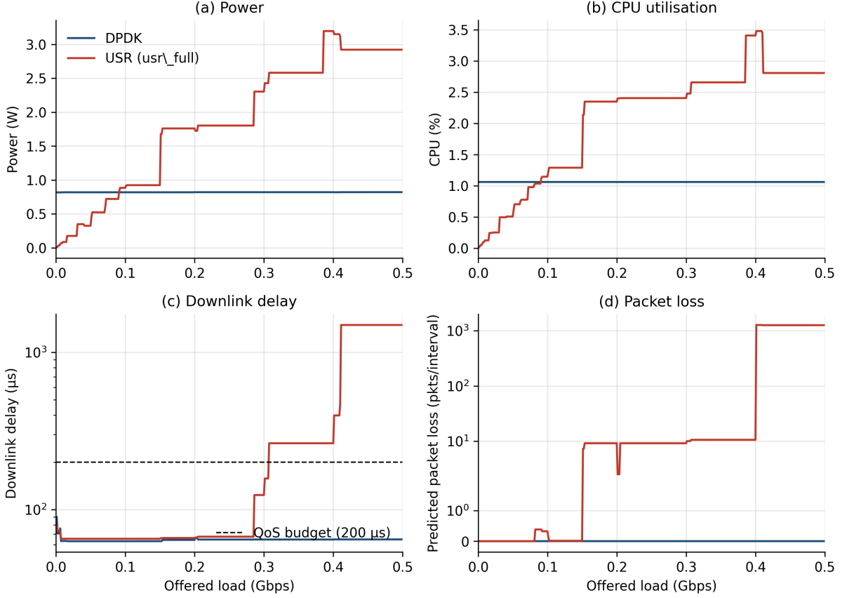
Figure 1.2: Twin-predicted UPF responses versus offered load (lite surrogate). (a) Power: SD-CORE DPKK flat near 0.82 W, USR-UPF rising and crossing SD-CORE DPKK at low load; (b) CPU; (c) downlink delay (log scale) with the 200 \mu s QoS budget marked; (d) predicted packet loss (symmetric-log scale). The USR-UPF staircase reflects the piecewise-constant nature of the tree-based lite models.
