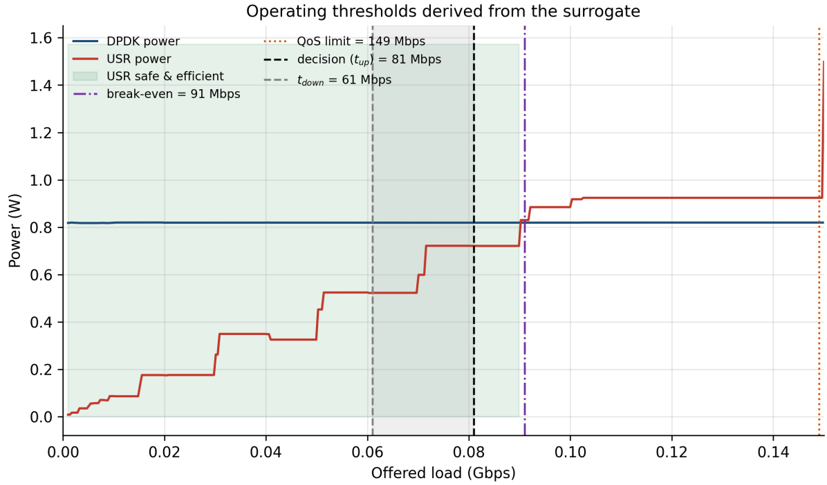
Figure 1.4: Operating thresholds derived from the surrogate. USR-UPF power (red) crosses SD-CORE DPDK power (blue) at the energy break-even (91 Mbps); the QoS limit (149 Mbps) is where USR-UPF first becomes unsafe. The decision threshold \lambda_{\uparrow} = 81 Mbps is the binding (energy break-even) limit minus a 10 Mbps margin; the shaded band down to \lambda_{\downarrow} = 61 Mbps is the hysteresis region. The green region marks loads where USR-UPF is both safe and cheaper than SD-CORE DPDK.
