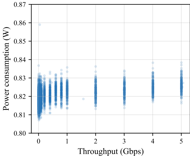
SD-Core DPDK
