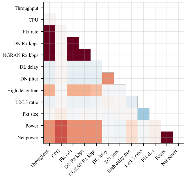
SD-Core DPDK
