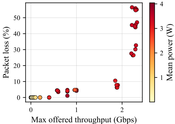
(a) Loss vs offered load
