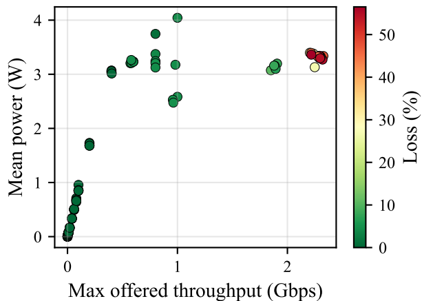
(b) Power vs offered load
