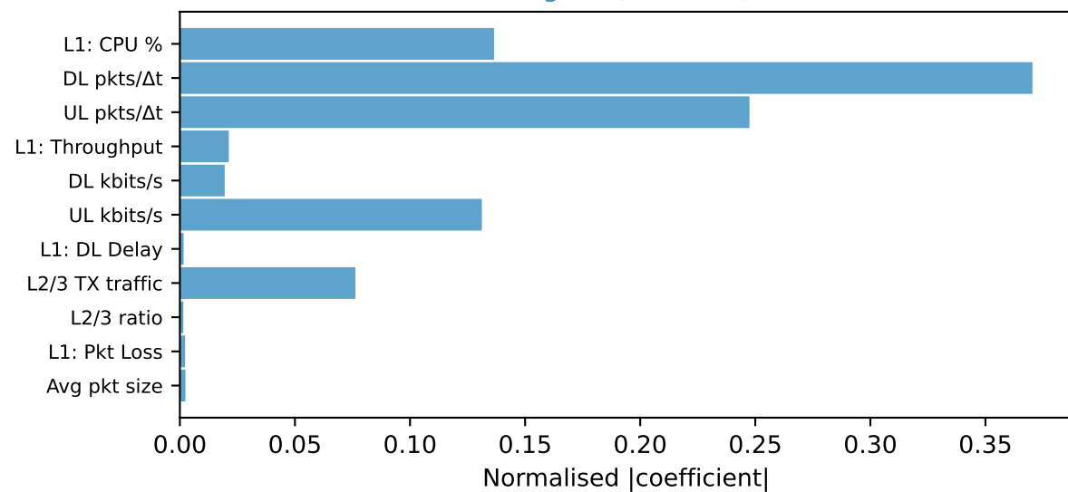
Ridge ★ ( R^2=0.999 )
