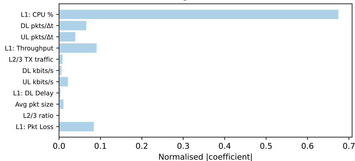
Ridge ★ ( R^2=0.999 )
