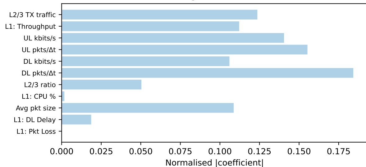
Ridge ( R^2=0.982 )
