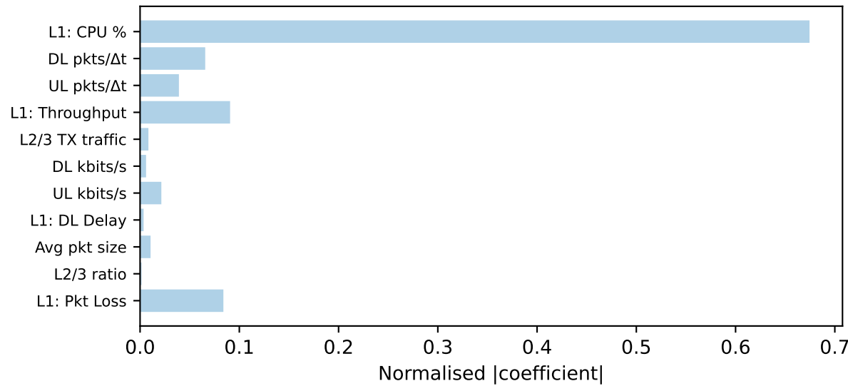
Ridge ★ ( R^2=0.999 )
