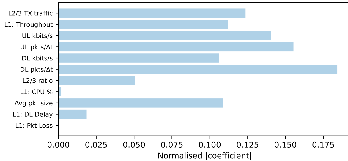
Ridge ( R^2=0.982 )
