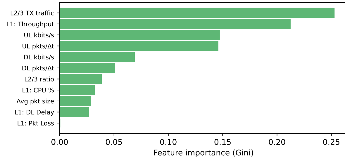
Random Forest ★ ( R^2=0.988 )
