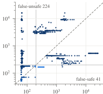
Mean DL delay ( \mu s)
