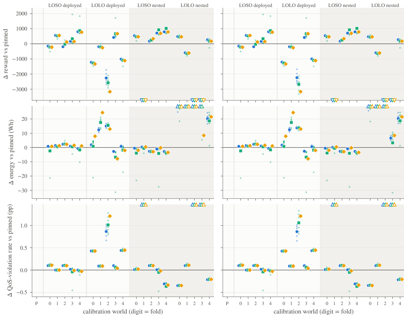
Experiment A — closed-policy zero-shot
