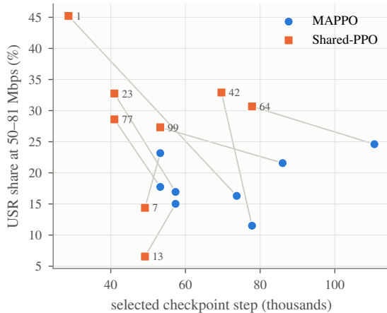
(b) Selection step vs USR use; lines join seeds
