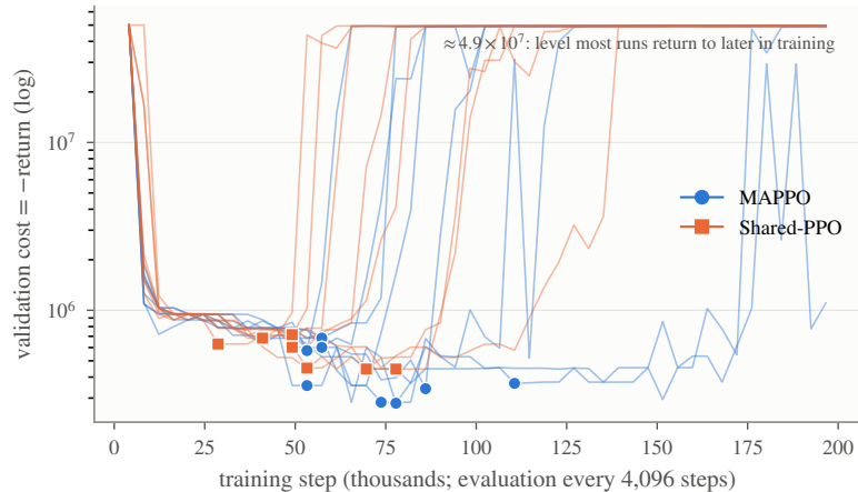
(a) Validation return during training; marker = selected checkpoint
